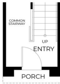
ELEVATION 2Z FIRST FLOOR (SAME AS ELEVATION 2X)
