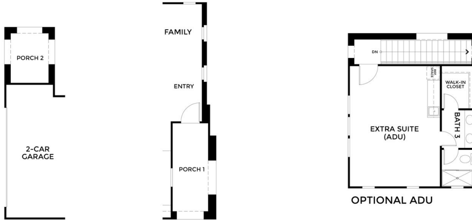
FIRST FLOOR ELEVATION C
