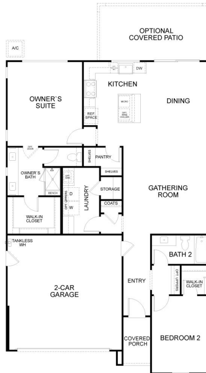
Floor Plan
